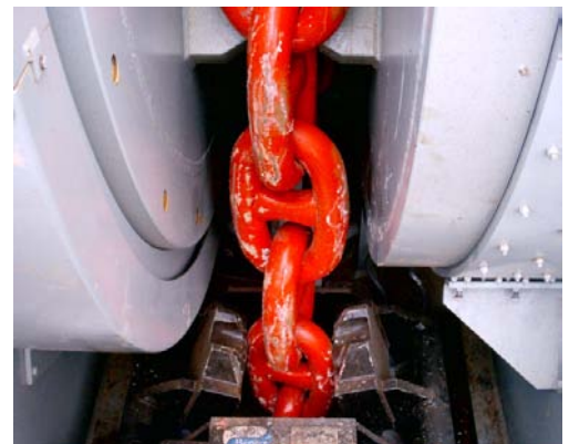
Dual Pawl Chain Stopper for 3-3/4" Chain
